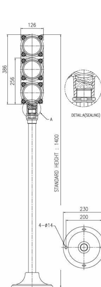
Standing Type
